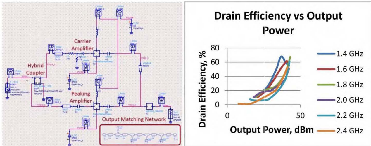
Figure 1. Class J-Tuned Doherty Amplifier Schematic (left), Drain Efficiency vs Output Power (right)
